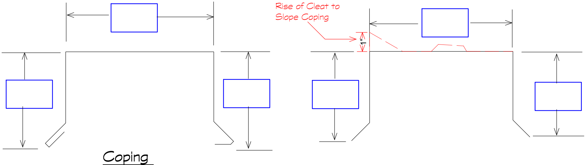
Coping Cleat And/Or Splice Plate
