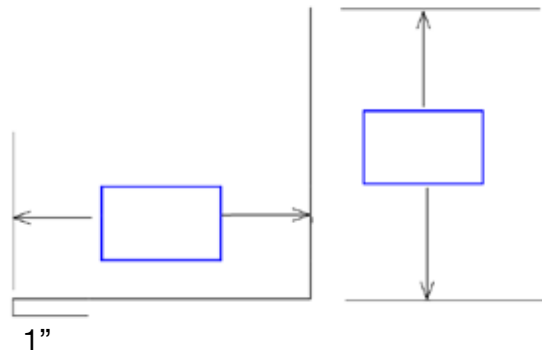
Side Wall Flashing
