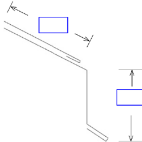
Drip Edge with Starter Cleat
